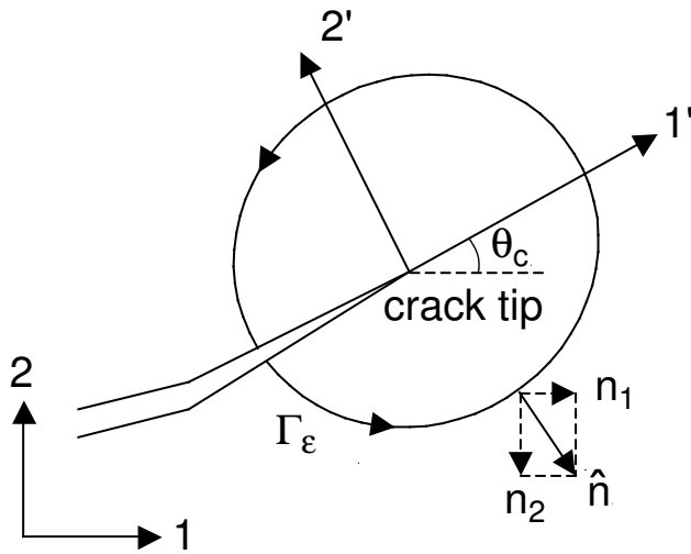
Figure 2 : Nomenclature and coordinates for terms used in the J -integral calculation. The 1 and 2 axes are global x and y axes. The 1' and 2' axes are aligned with the current crack direction. The contour \Gamma_\varepsilon starts on one crack surface and proceeds counter-clockwise to the opposite crack surface.
