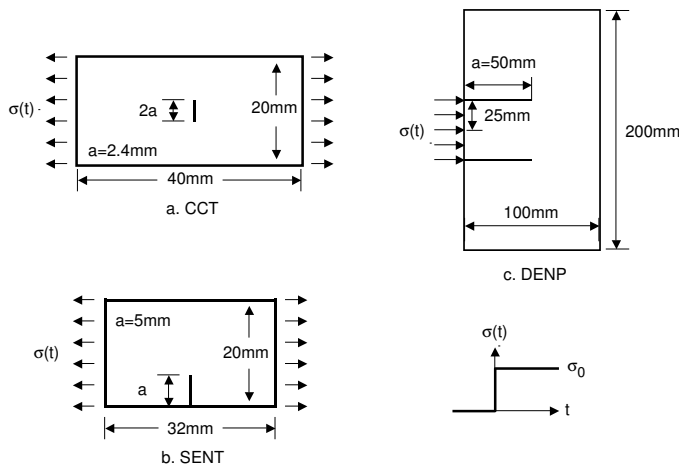
Figure 7 : Specimen geometries for dynamic stress intensity factor calculations. a. Center crack tension (CCT) specimen. b. Single edge notched tension (SENT) specimen. c. Double edge notched plate (DENP) specimen. All specimens were loaded (as indicated by arrows) instantaneously at time zero and then the stress was held constant.
