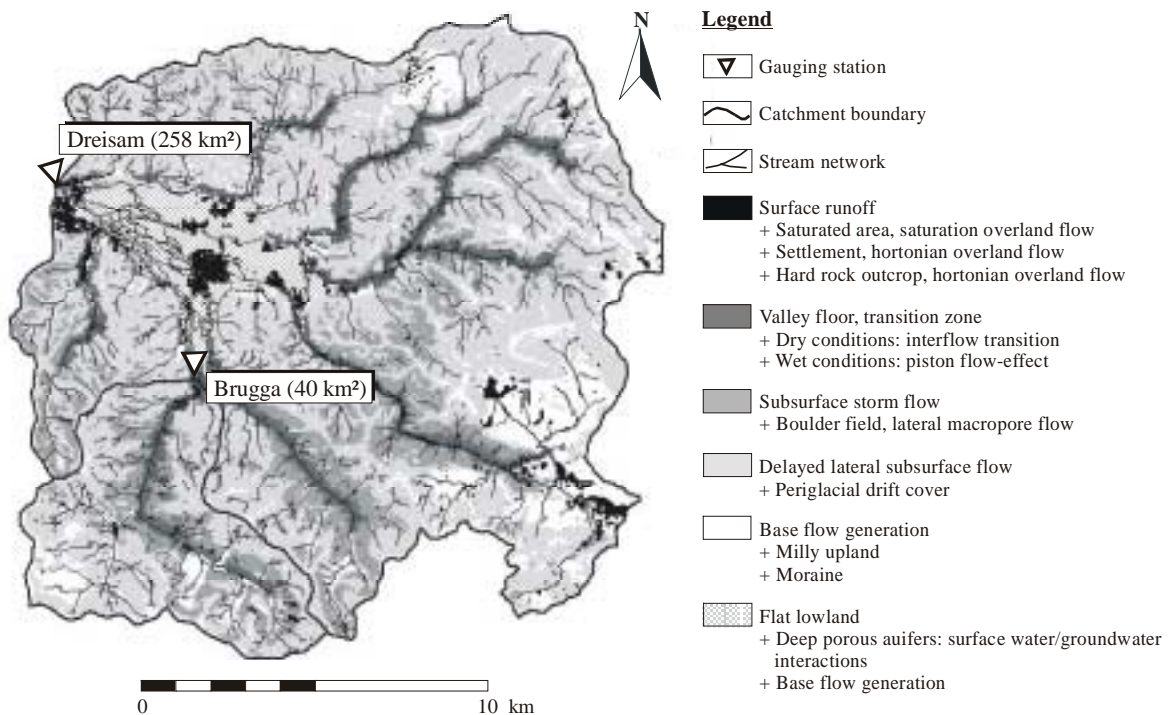
Fig. 1: Landscape units with the same dominating runoff generation processes (described in the legend) at Dreisam basin (Black Forest Mountains, south-west Germany). The highly investigated sub-basin Brugga is located in the southwest.
