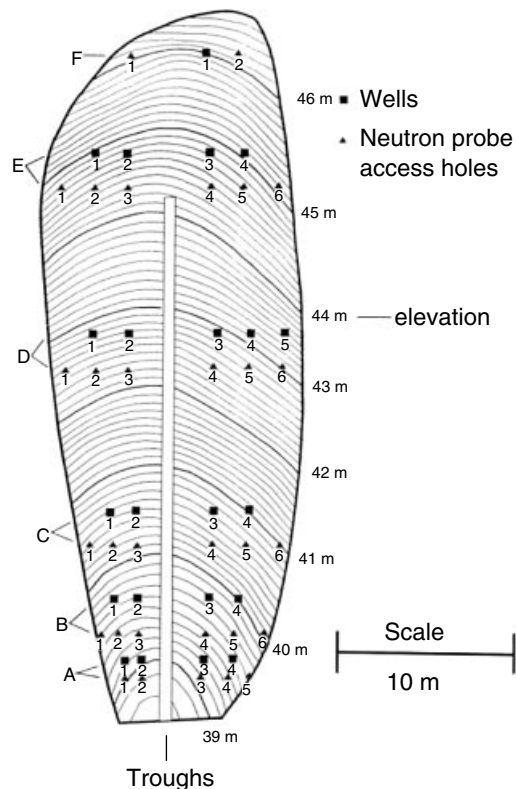
Figure 1. Plan view of the surface topography of the Hydrohill #2 experimental catchment showing the locations and numbers of wells and neutron probe access holes, and the central stacked lysimeter troughs. The numbers to the left of the map indicate the row number, e.g. well number 1 of row D is well D1, etc
