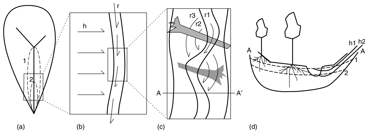
Figure 1. Conceptual model of vegetation–hydrology coupling at diel time scales over the summer baseflow recession period in a headwater basin (Watershed 1) in the H.J. Andrews Forest. (a) The basin consists of hillslopes and the valley floor, including the stream channel and floodplain/terraces, the groundwater system and the riparian system. (b) Hydrologic flowpaths operate on hillslopes (h) and in the riparian zone (r). (c) Riparian zone flowpaths include in-streamflow (r1), near-stream, fast, hyporheic exchange flowpaths (r2), and far-from-stream, slow, hyporheic exchange flowpaths (r3), created by sediment and large wood stored in the valley floor. (d) A cross-section of the valley floor shows shallow flowpaths (h1) and deep flowpaths on hillslopes (h2) contributing lateral flow to the valley floor and stream, and the changing positions of a water table or near-saturated zone in early summer (time 1) and late summer (time 2). The vegetation zone of influence on the diel cycles in streamflow can be envisioned as an area of lower hillslopes and the riparian zone (a) with a water table at a given height (1 or 2 in (d)). In early summer, when the water table is high (time 1), the stream channel has surface flow (r1) and is exchanging flow actively with the hyporheic zone through near-streamflowpaths (r2, part (c)). At time 1, the water table, or some near-saturated zone, is within the reach of most roots of riparian and lower hillslope vegetation (d). Thus, water use by lower hillslope and riparian vegetation produces a local depletion of moisture at the time of maximum sapflow, which is measured as a daily minimum in streamflow at some later time that day. The time lag between maximum sapflow and minimum streamflow is relatively short, because water routing through the flowpaths involved (h1, r1 and r2, parts (c) and (d)) is relatively fast. Later in the summer (time 2), when the water table has fallen, the stream channel has less surface flow and less active exchange along short hyporheic flowpaths, so the contributions of h1, r1 and r2 to streamflow are diminished relative to h2 and r3 (parts (c) and (d)). At time 2, the water table and near-saturated zone fall below the reach of most roots of riparian and lower hillslope vegetation (d). As in the early summer, local depletion is transmitted to the stream gauge through predominantly slower flowpaths (such as r3, part (c)), lengthening the time lag between maximum sapflow and minimum streamflow. Also, because deep flowpaths beyond the reach of tree roots are relatively more important to streamflow in late summer, the strength of the relationship between maximum sapflow and minimum streamflow declines at time 2 relative to time 1. By very late summer, the increasing dominance of deep hillslope and long hyporheic flowpath contributions to streamflow obscure the connection between sapflow and streamflow, almost eliminating the diel cycle in streamflow. These changes may be associated with a contraction of the area of vegetation influence from time 1 to time 2 (part (a))
