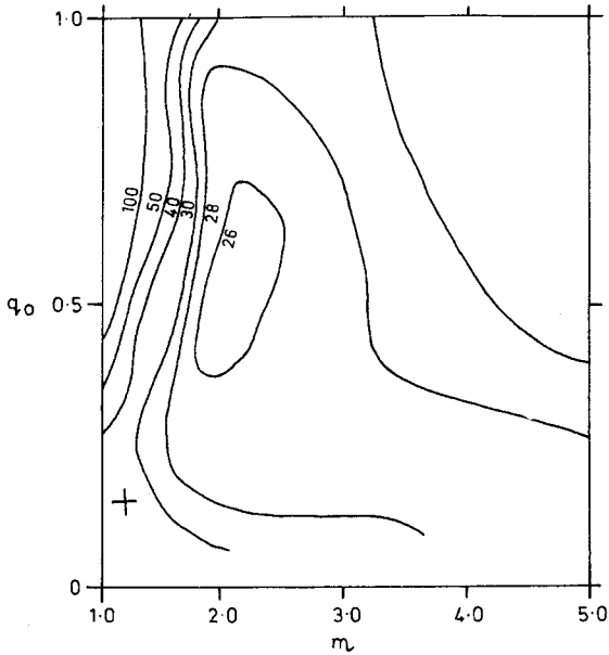
FIG. 14. F_1 response surface for the parameters m and q_0 . Lanshaw sub-basin November/December 1974 simulation. Cross represents estimated values.
