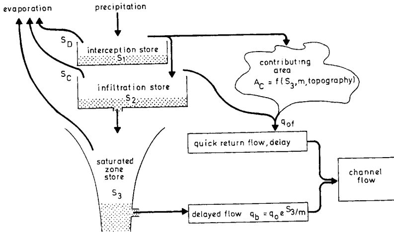
FIG. 1. A schematic representation of the sub-basin model.
