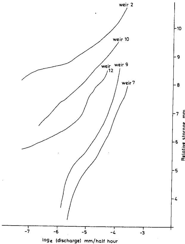
FIG. 8. Recession curves for different sites in the Crimble Beck basin as storage/ \ln (discharge) plots.
