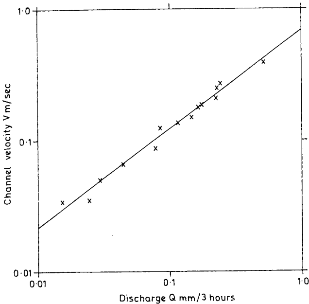
FIG. 10. Plot of average channel flow velocity measured by dilution gauging at a site in the centre of the basin, against discharge from Crimple Beck.
