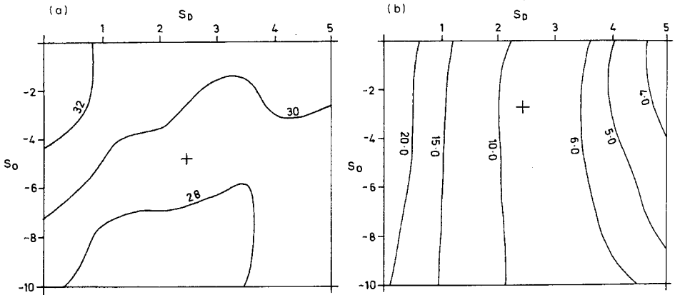
FIG. 15. (a) F_1 response surface for the parameters S_D and S_0 . Lanshaw sub-basin, November/December 1974 simulation. Cross represents estimated values. (b) F_1 response surface for the parameters S_D and S_0 . Lanshaw sub-basin, March/April 1975 simulation. Cross represents estimated values.
