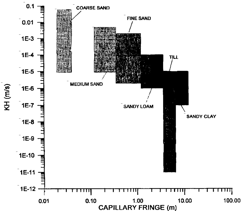
Fig. 2. Envelopes encompassing relationships between height of the capillary-fringe (from Zaltsberg, 1986) and saturated hydraulic conductivity ( K_H ) (from Freeze and Cherry, 1979 and Domenico and Schwartz, 1990) for various geologic materials.
